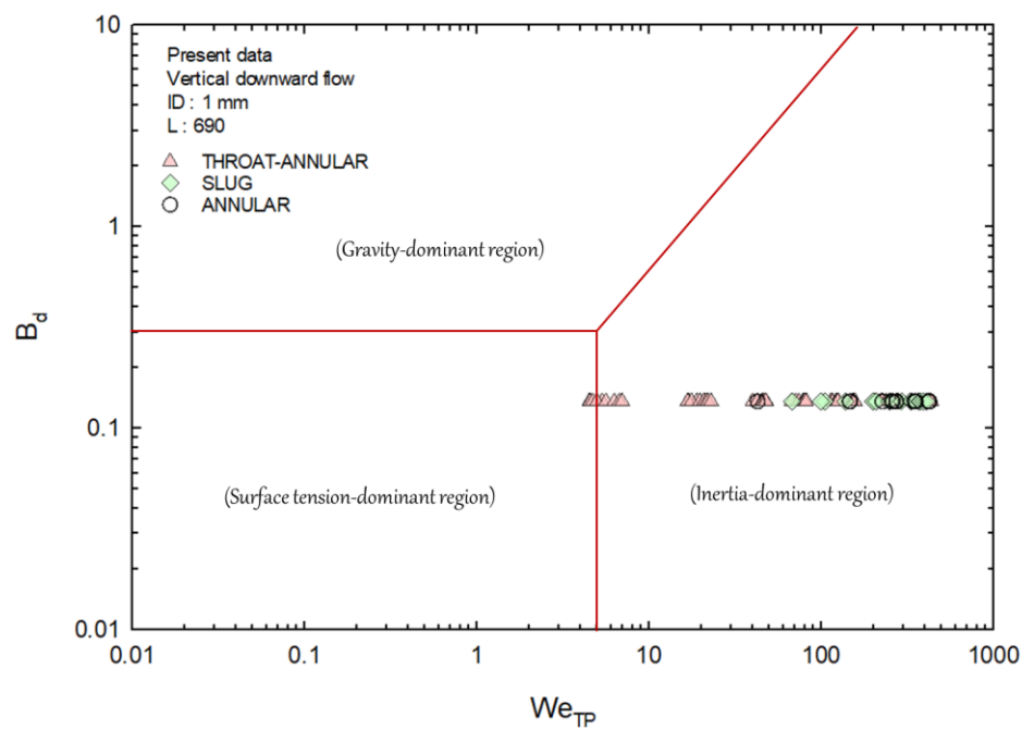
Figure 4 Force regime map from vertical downward flow
