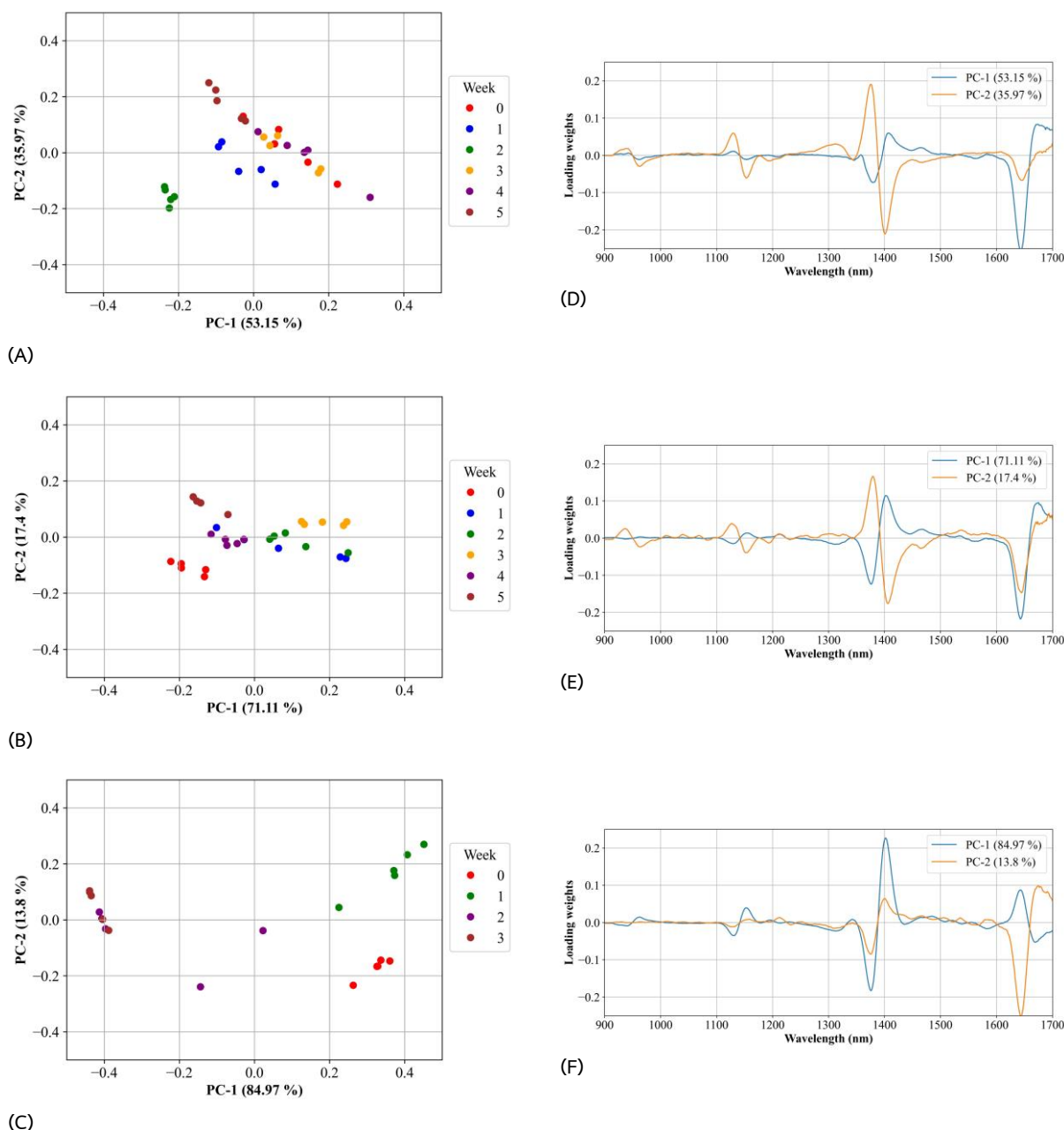
Figure 6 The PCA Score plot (A-C) and Loading plot (D-F) of NIRs spectral data from center leaves (P2) treatment of control (T0) (A, D), treatment for non-fertilized, watered seedlings (T1) (B, E) treatment for non-watered, fertilized seedlings (T2) (C, F).
